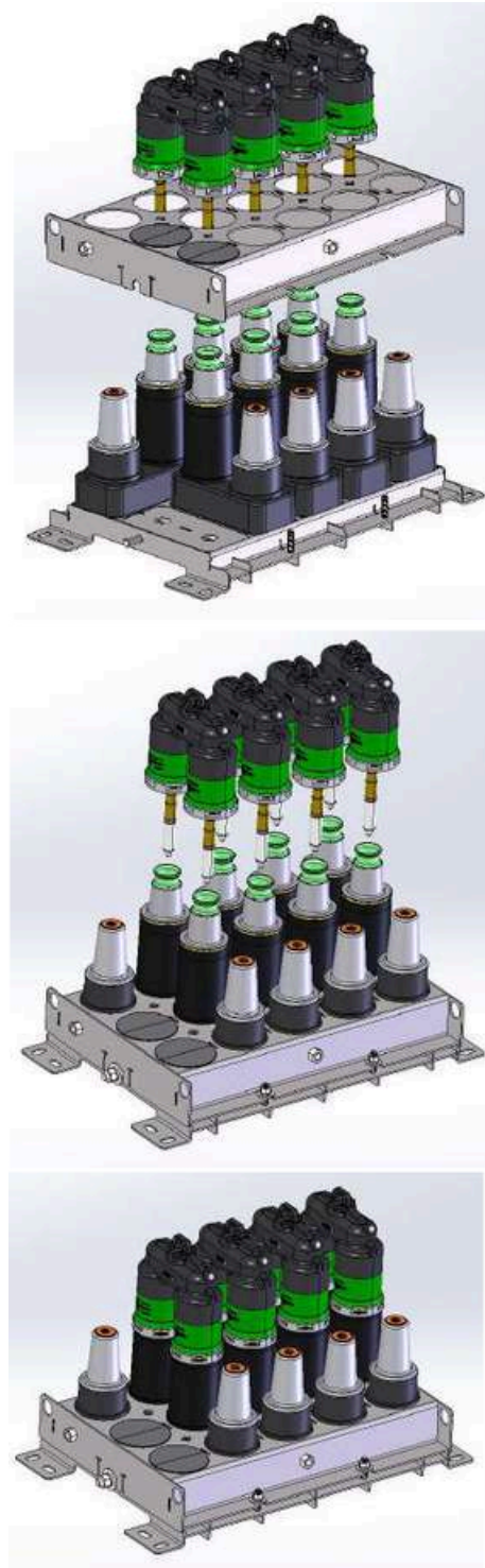
Figure 5. Exploded view of Cleer multi-point junction assembly demonstrating use of multiple junction buss, bracket and C-connectors to make full switching assembly.
