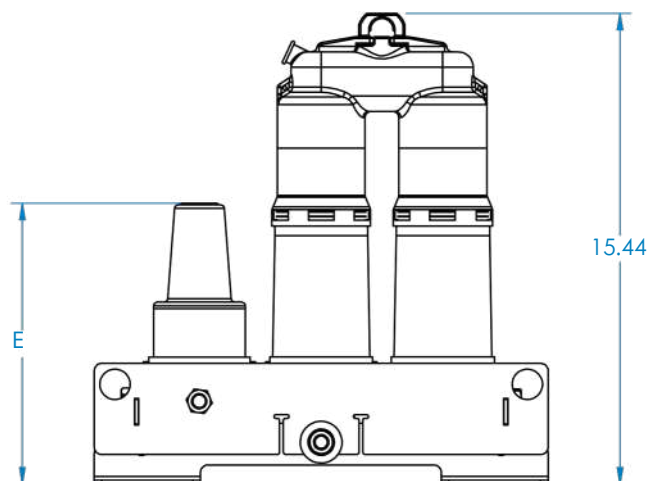
Figure 8. Cleer multi-point variable junction assembly - side view.
